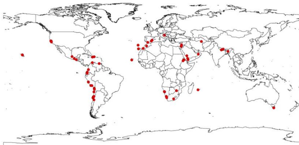
Fig. 8 Locations where fog collection has a high potential for success (adapted from Klemm et al. 2012)
