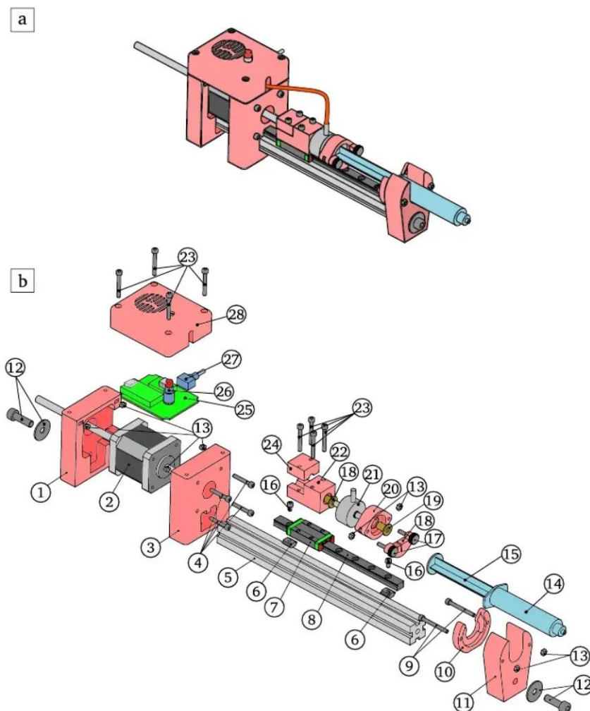
Fig. 3. a) Ystruder assembly, 3D printed parts shown in red color b) Exploded view of the Ystruder assembly with part numbering using the same color scheme. For associating numbers with respective component names, the reader is referred to the web version of this article.
